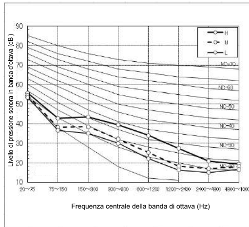
MMK-UP0181HP(L)*
