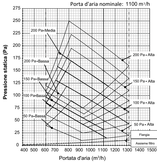
MMD-UP0271HP-E / TR
