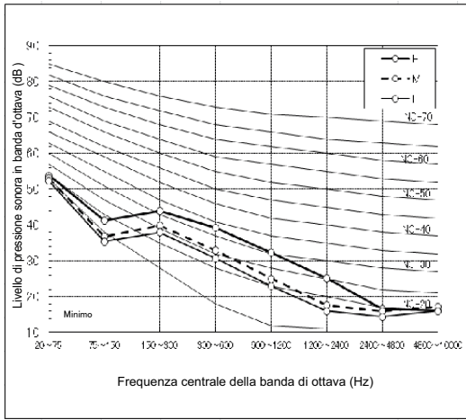
MMK-UP0151HP(L)*
