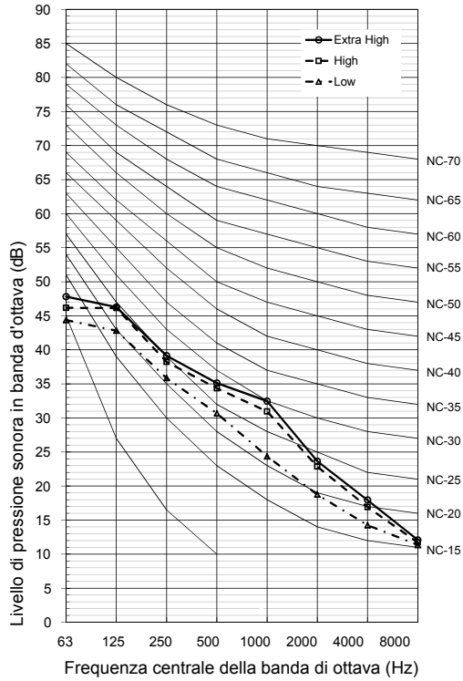
VN-M1000HE1
