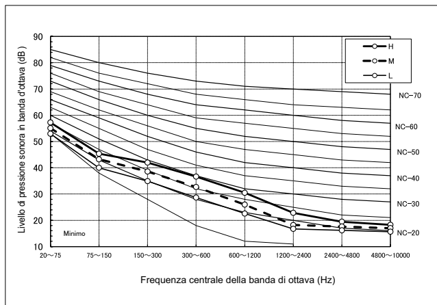
MMK-UP0151HP(L)*
