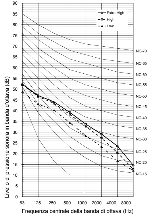
VN-M1500HE1
