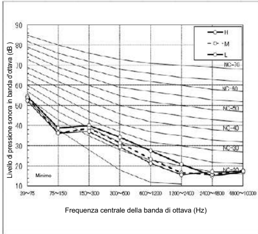
MMK-UP0091HP(L)*
