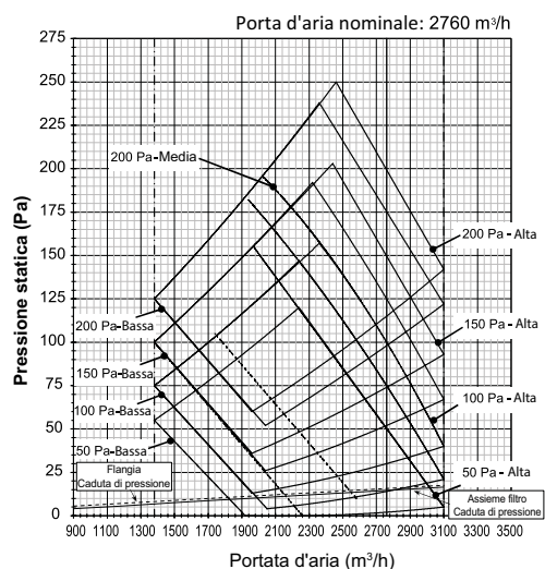
MMD-UP0561HP-E / TR
