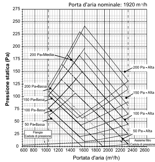
MMD-UP0561HP-E / TR
