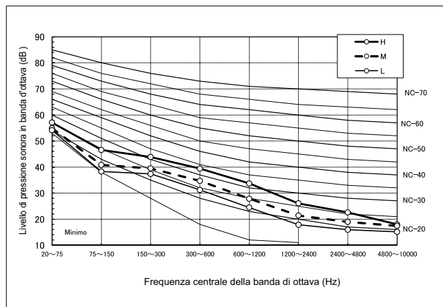
MMK-UP0181HP(L)*
