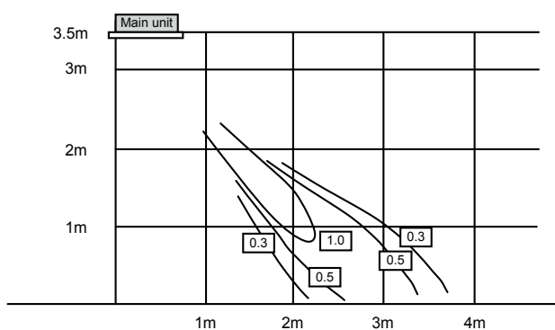
MMU-UP0151SH-E, UP0181SH-E
