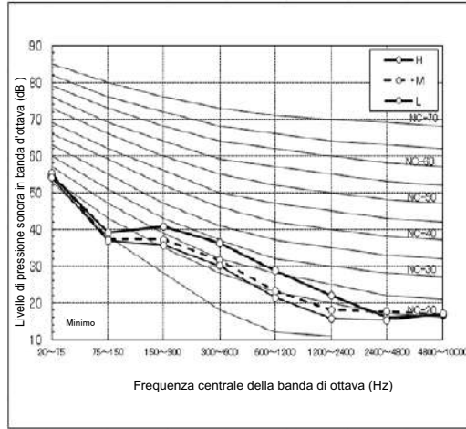
MMK-UP0121HP(L)*
